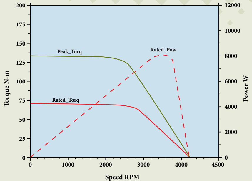
M22B2 Performance Data
