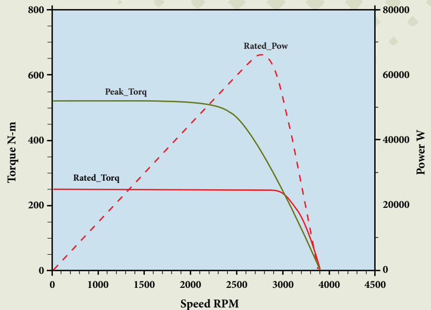
M40B2 Performance Data
